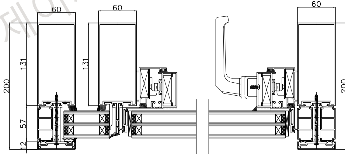
2 HORIZONTAL SECTION (B-B')
