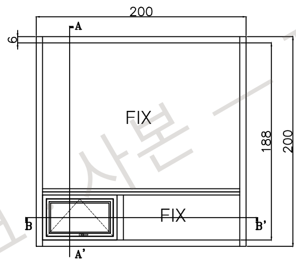
ELEVATION (INSIDE VIEW)
